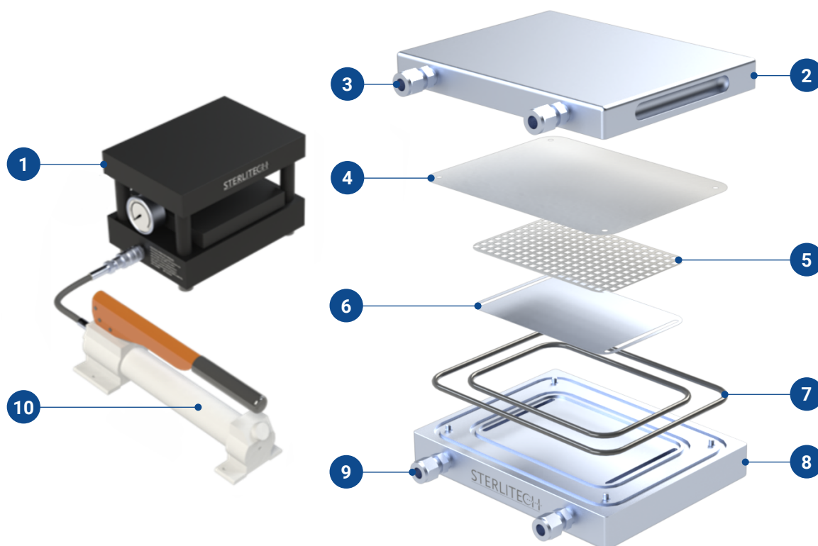
Figure 1: Hastelloy Sepa FO Cell Assembly
