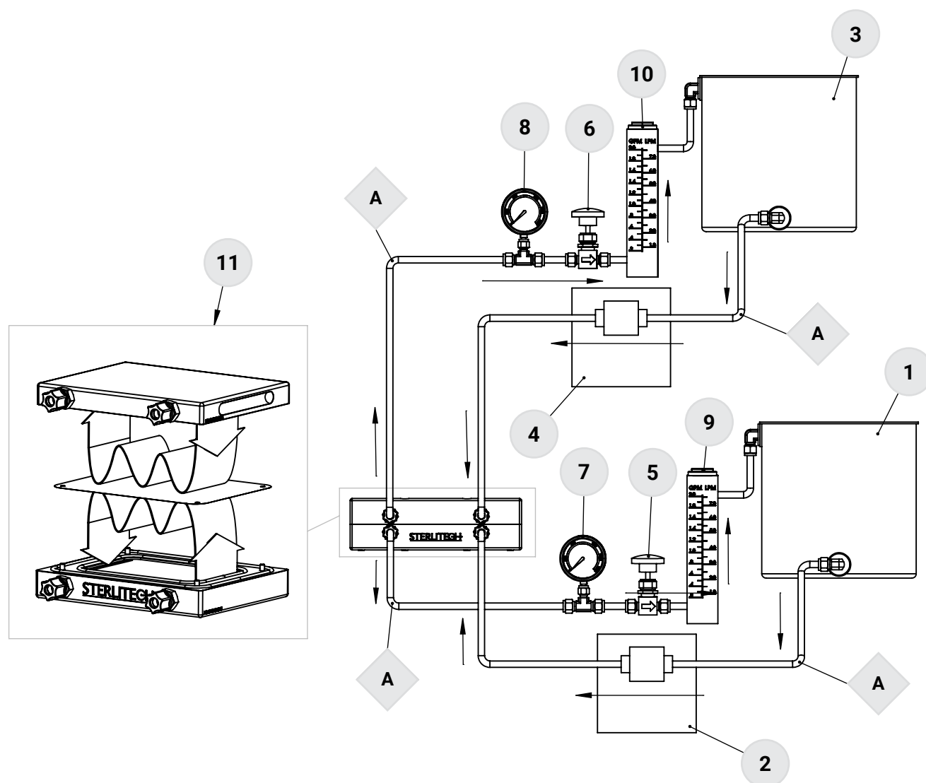
Figure 2: Forward Osmosis System Diagram for Hastelloy Sepa FO Cell
