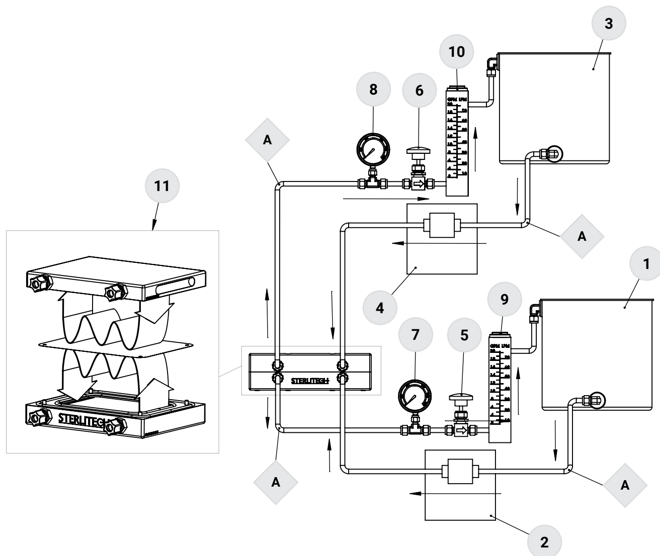
Figure 2: Forward Osmosis System Diagram for 316SS Sepa FO Cell
