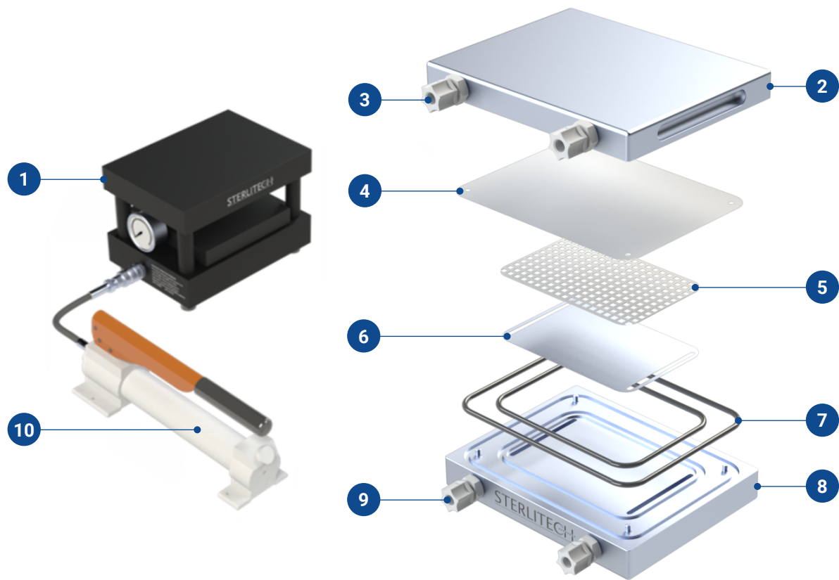
Figure 1: 316SS Sepa FO Cell Assembly
