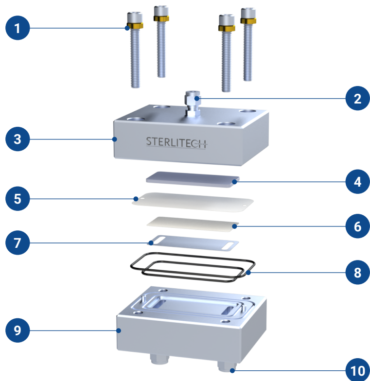
Figure 1: CF042H Crossflow Cell Body Assembly
