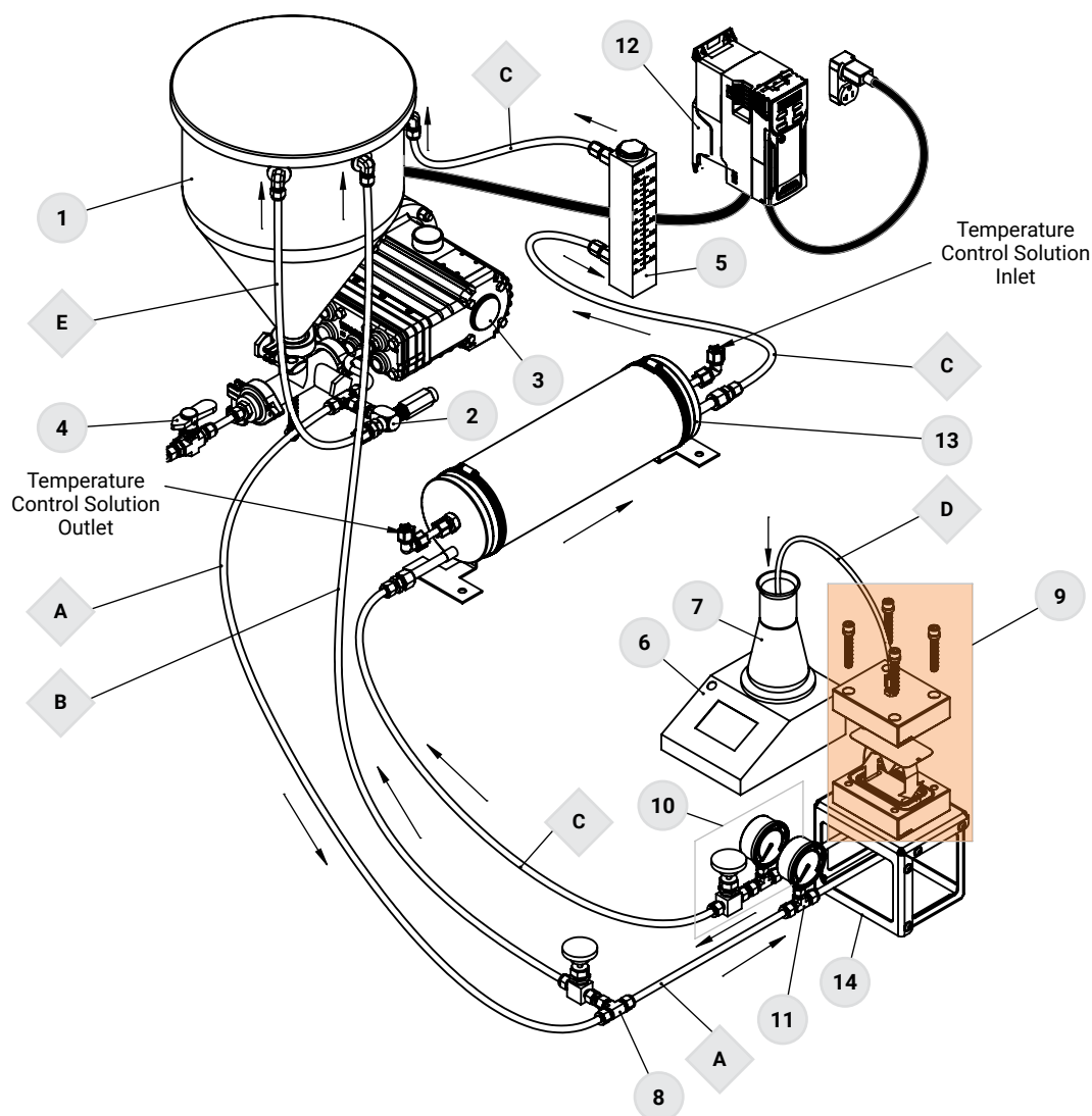
Figure 2: Cross Flow System Diagram for CF042H Cell
