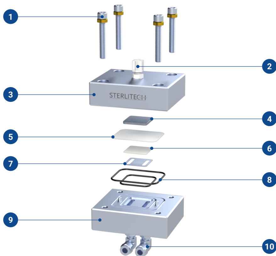
Figure 1: CF016SS Crossflow Cell Body Assembly
