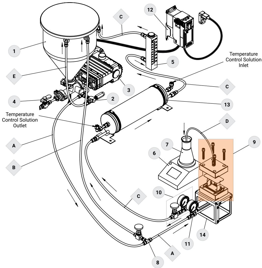
Figure 2: Cross Flow System Diagram for CF016SS Cell
