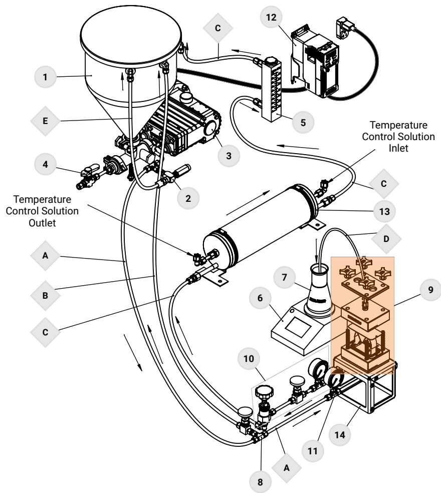
Figure 2: Cross Flow System Diagram for CF016P Cell
