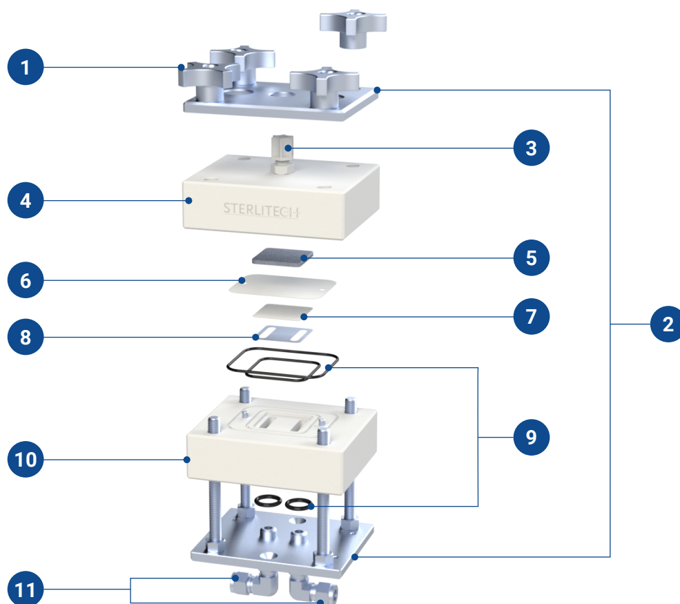
Figure 1: CF016P Crossflow Cell Body Assembly
